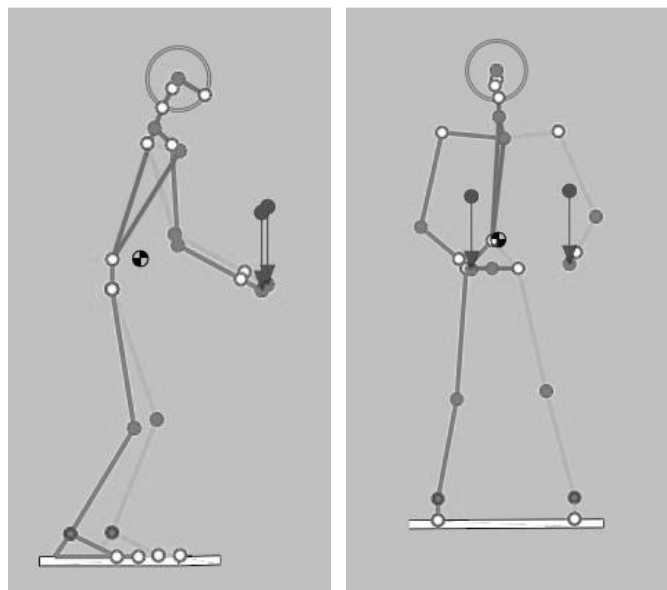
Fig. 6. Position 3. Position adopted when moving a concrete block. Edge views from the side and front
